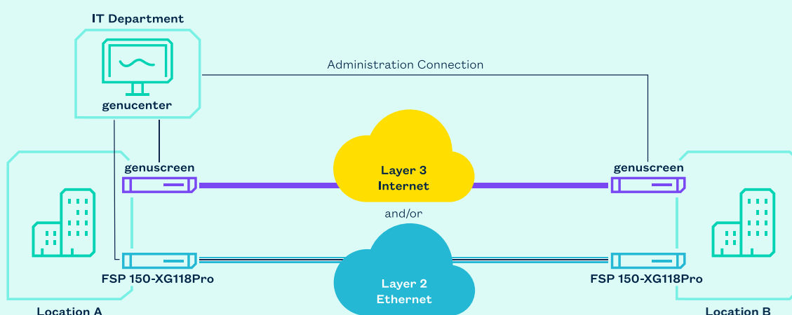
Network-layer 2/layer 3 encryption with integrated administration capability
