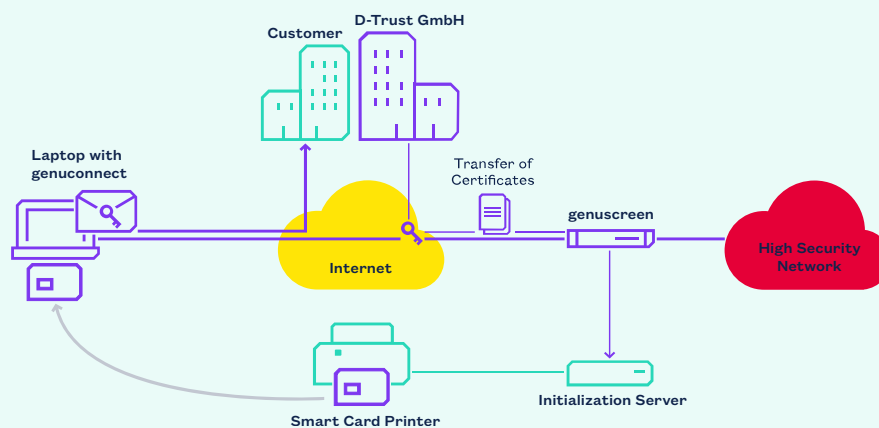
Ecosystem for classification level German VS-NfD with VPN software client and Certificate Solution genustrust
