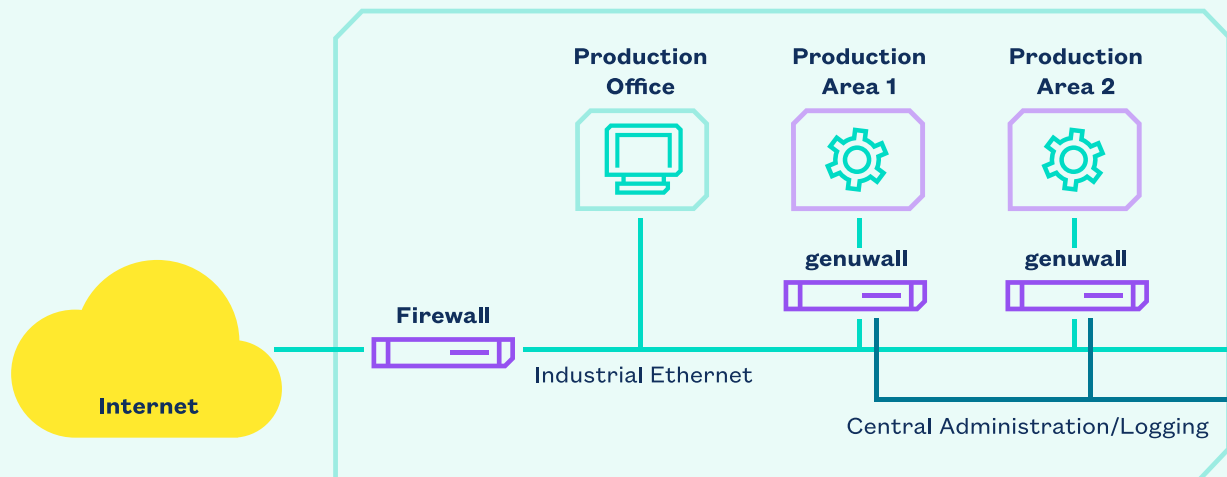
Segmentation for secure production areas with genuwall.
