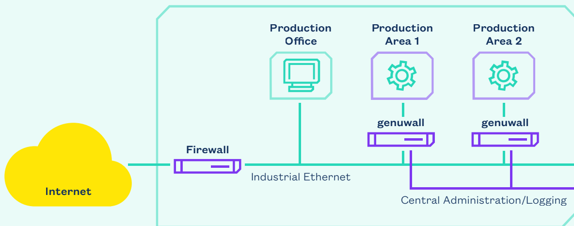
Segmentation for secure production areas with genuwall
